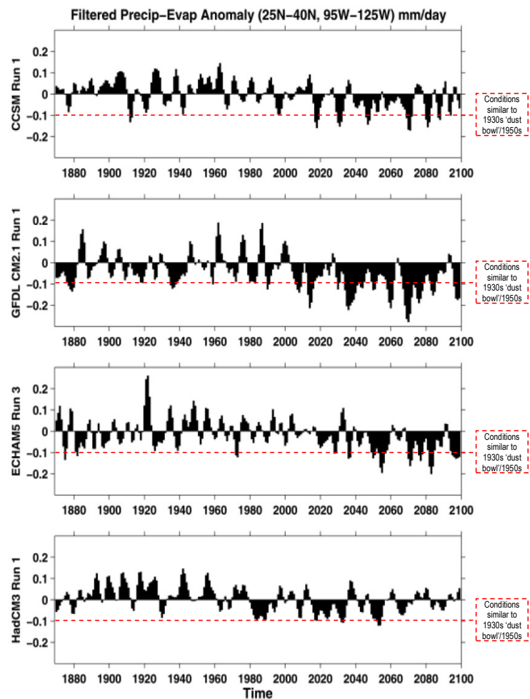
Figure 3.5.2: Change in annual mean P – E over the American Southwest for four coupled models
