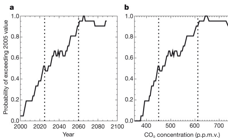
Figure 3.4.5: Predicted change in the probability of a 2005-like drought in Amazonia, based on results from the HadCM3LC GCM run with aerosols 11 (after Cox et al, 2008 (3))
