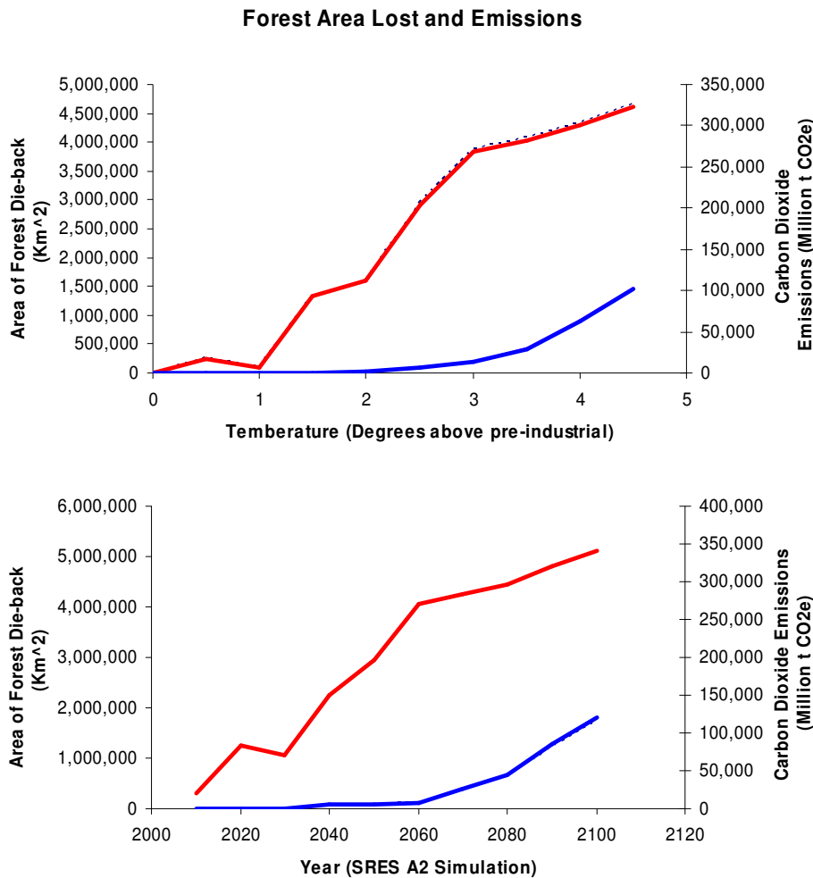
Figure 3.4.3: Forest Area lost and CO 2 emissions
