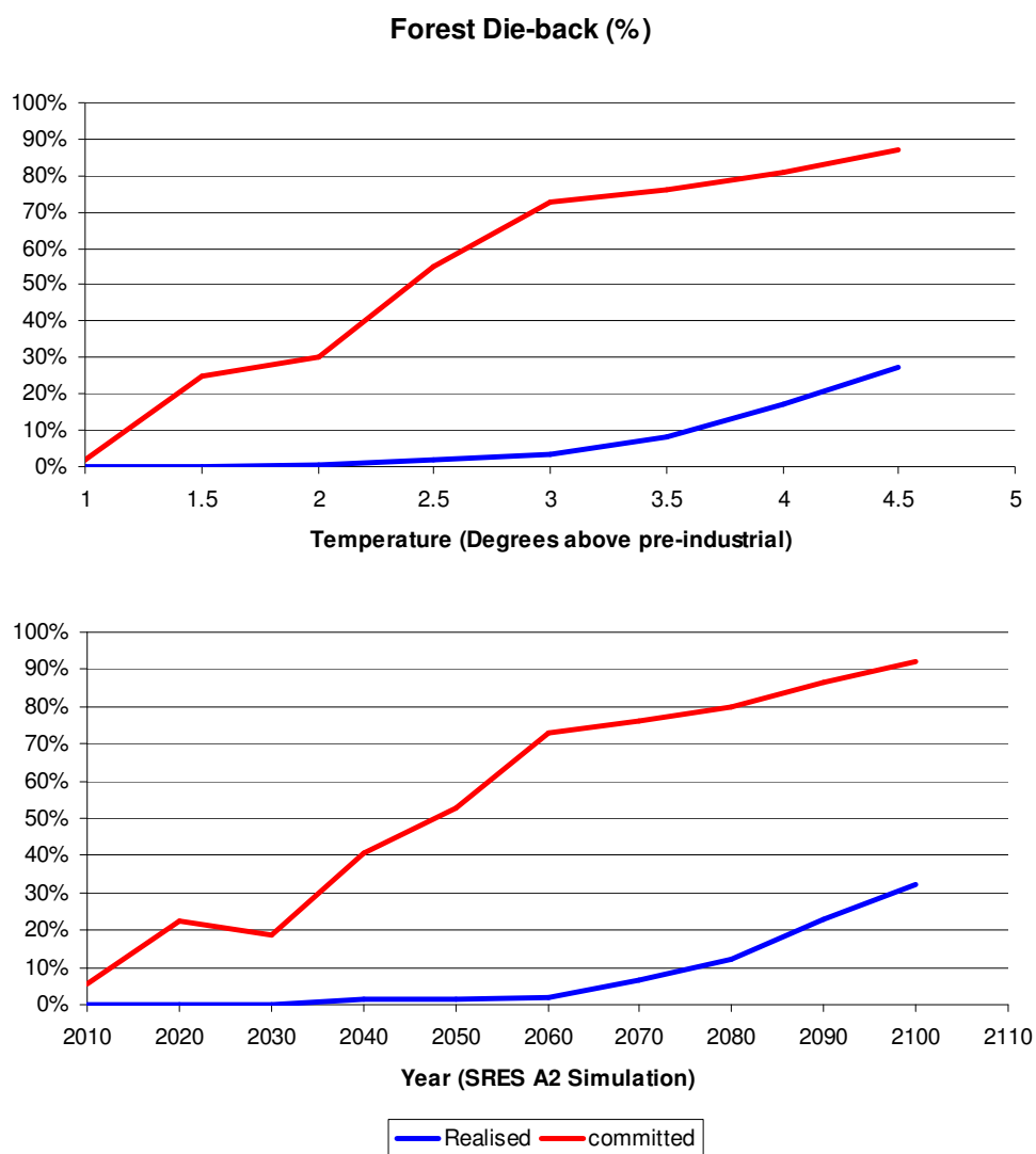
Figure 3.4.1: Realised and committed dieback of the Amazon rainforest – after Jones et al (2009) (37)
